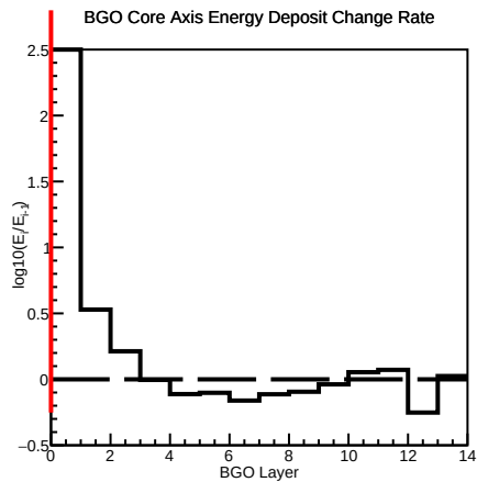
BGO Core Axis Energy Deposit Change Rate
