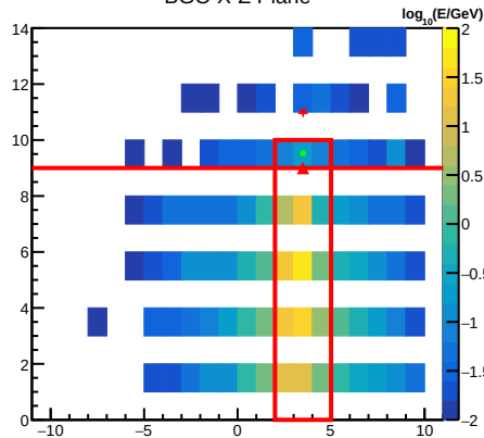
BGO Core Axis Energy Deposit
