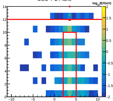
BGO Y-Z Plane
