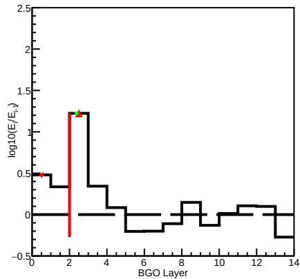
BGO Core Axis Energy Deposit Change Rate
