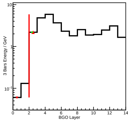
BGO Core Axis Energy Deposit
