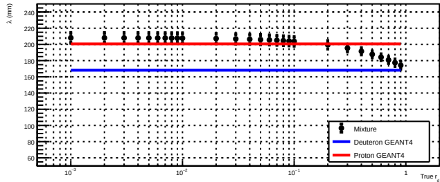
Fitted From N_{\text{int}}
