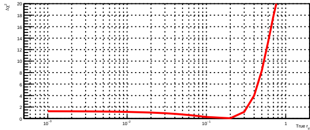
Fitted From N_{\text{sur}}
