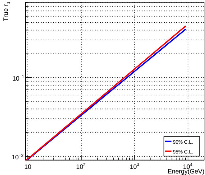
Sensitivity Curve from N_{\text{int}}
