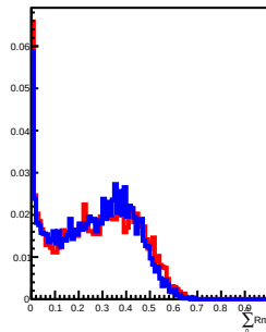
1000 GeV incident in L11
