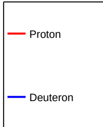
IncidentParticle 1000GeV
