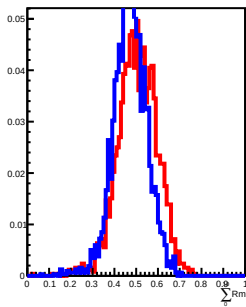
100 GeV incident in L10
