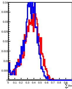
100 GeV incident in L11
