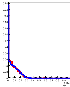
100 GeV incident in L7
