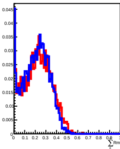
100 GeV incident in L9
