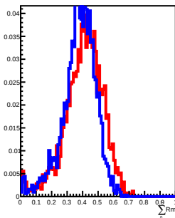
100 GeV incident in L12
