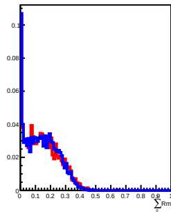
100 GeV incident in L8
