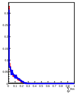
200 GeV incident in L7
