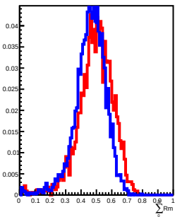
200 GeV incident in L9
