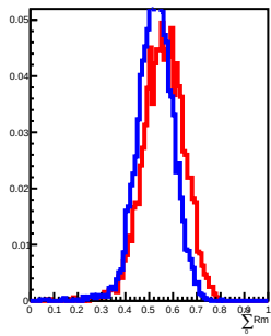
200 GeV incident in L11
