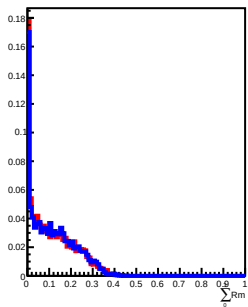
200 GeV incident in L8
