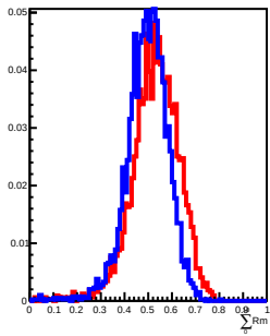
200 GeV incident in L10
