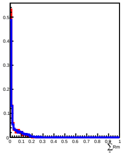
20 GeV incident in L5
