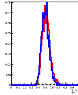
20 GeV incident in L13
