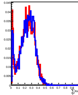
20 GeV incident in L8
