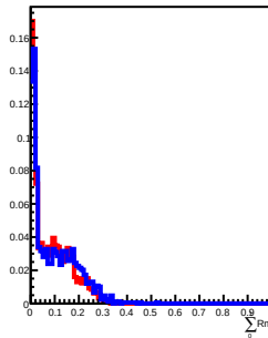
20 GeV incident in L6
