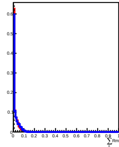
300 GeV incident in L6
