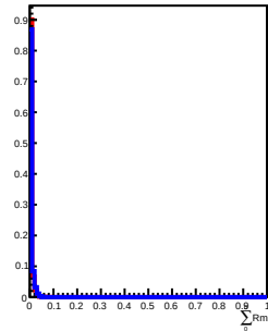
300 GeV incident in L5
