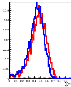
300 GeV incident in L13
