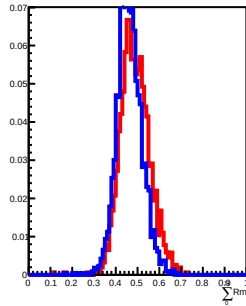
30 GeV incident in L11
