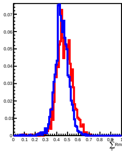
30 GeV incident in L10
