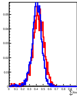
30 GeV incident in L13
