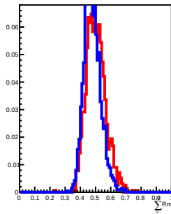
30 GeV incident in L12
