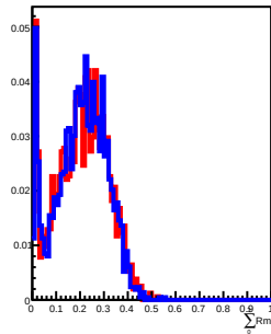
30 GeV incident in L8
