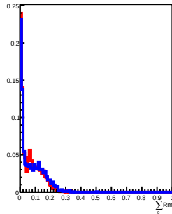
30 GeV incident in L6
