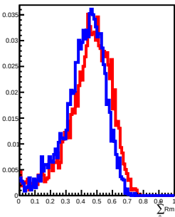
400 GeV incident in L13
