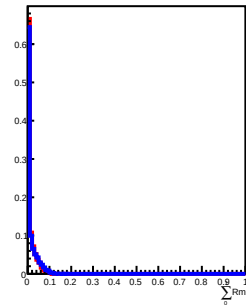
400 GeV incident in L6
