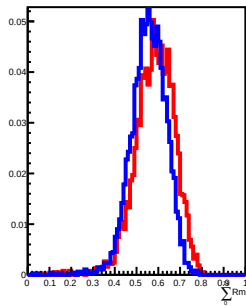
400 GeV incident in L11
