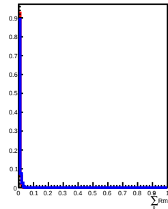
400 GeV incident in L5
