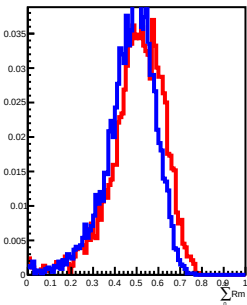
400 GeV incident in L9
