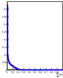
400 GeV incident in L7
