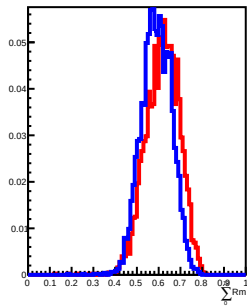
400 GeV incident in L12
