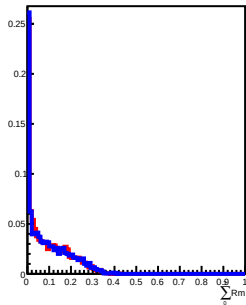
400 GeV incident in L8
