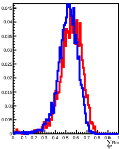
400 GeV incident in L10
