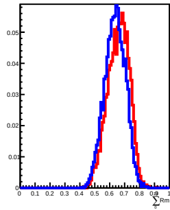
500 GeV incident in L13
