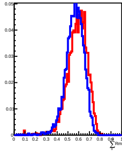
500 GeV incident in L11
