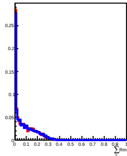
500 GeV incident in L8
