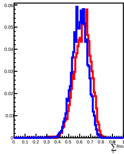
500 GeV incident in L12
