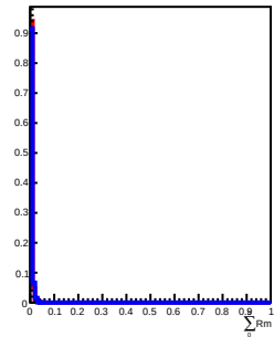
500 GeV incident in L5
