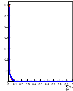
500 GeV incident in L6
