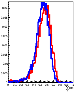
500 GeV incident in L10
