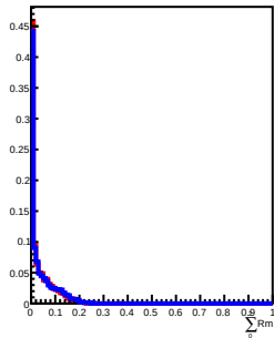
500 GeV incident in L7
