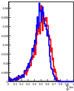
500 GeV incident in L9
