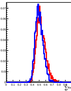
50 GeV incident in L13
