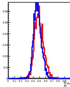
50 GeV incident in L11
