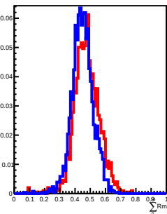
50 GeV incident in L10
