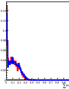
50 GeV incident in L7
