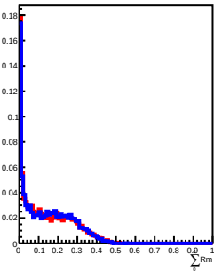
600 GeV incident in L9
