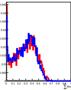
600 GeV incident in L11
