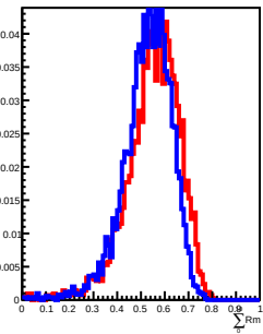
600 GeV incident in L10
