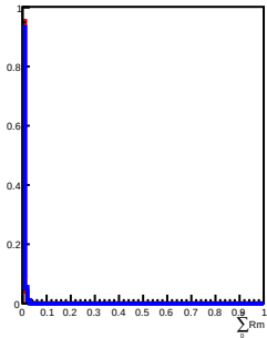
600 GeV incident in L5
