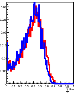
600 GeV incident in L12
