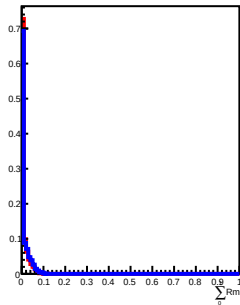
600 GeV incident in L6
