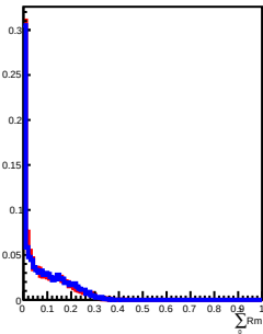
600 GeV incident in L8
