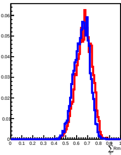
600 GeV incident in L13
