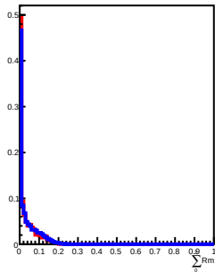
600 GeV incident in L7
