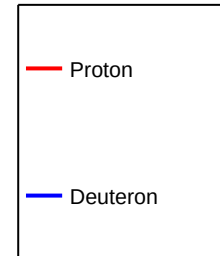
IncidentParticle 60GeV
