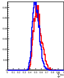
60 GeV incident in L13
