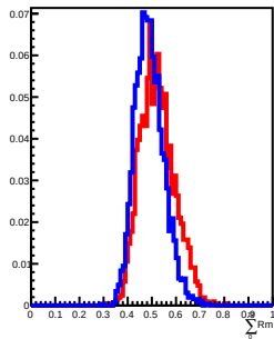
60 GeV incident in L12
