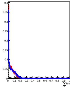
60 GeV incident in L6
