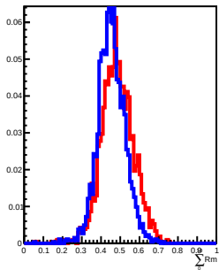
60 GeV incident in L10
