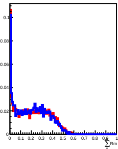
700 GeV incident in L10
