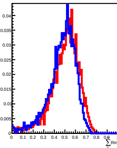
700 GeV incident in L9
