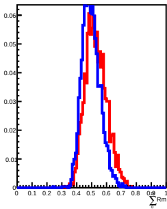
70 GeV incident in L12
