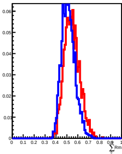
70 GeV incident in L13
