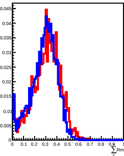
70 GeV incident in L10
