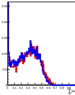
800 GeV incident in L11
