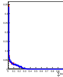
800 GeV incident in L8
