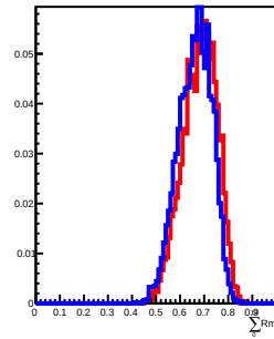
800 GeV incident in L13
