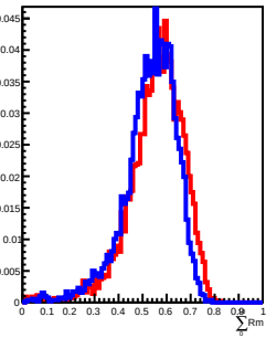
800 GeV incident in L10
