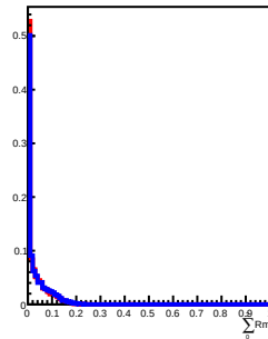
800 GeV incident in L7
