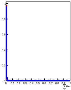
800 GeV incident in L5
