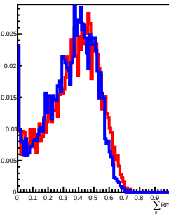
800 GeV incident in L12
