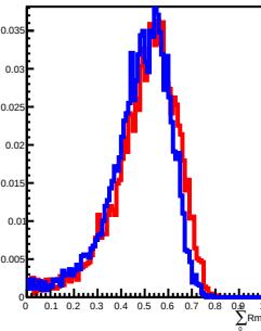
800 GeV incident in L9
