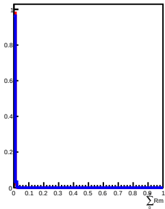
900 GeV incident in L5
