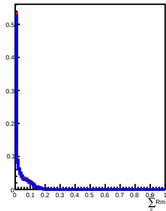
900 GeV incident in L7
