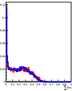
900 GeV incident in L10
