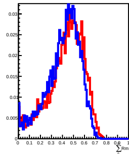
900 GeV incident in L13
