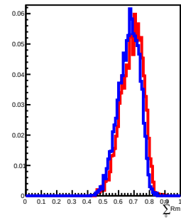
900 GeV incident in L13
