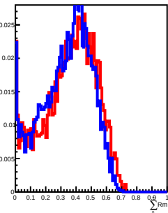
900 GeV incident in L12
