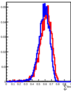
900 GeV incident in L11
