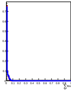
900 GeV incident in L6
