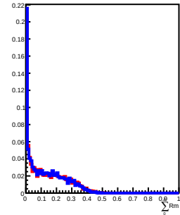
900 GeV incident in L9
