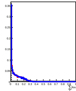
900 GeV incident in L8
