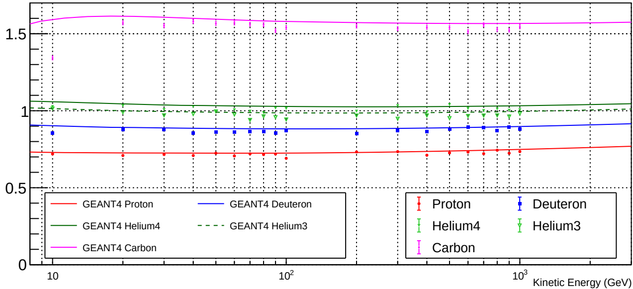
Fitted Hadronic Interaction Cross Section vs Energy
