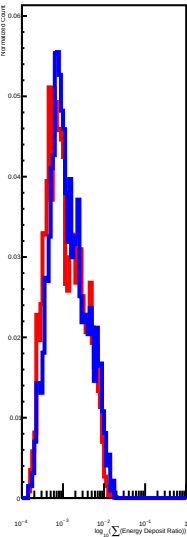
Distribution of \sum_{\sigma}^{L0} EdepRatio
