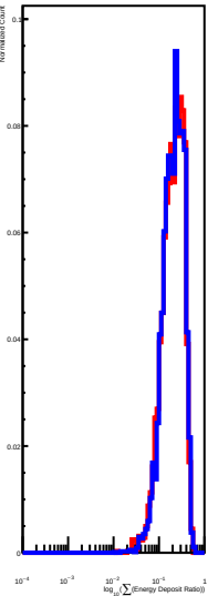
Distribution of \sum_{\sigma}^{L4} EdepRatio
