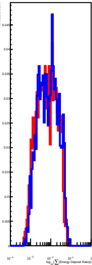
Distribution of \sum_{\sigma}^{L1} EdepRatio
