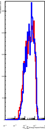
Distribution of \sum_{\sigma}^{L2} EdepRatio
