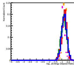
EdepRatio Distrubution in L1
