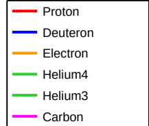
IncidentParticle 30GeV
