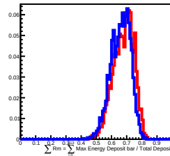
1000 GeV incident in L13
