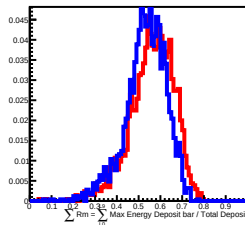
1000 GeV incident in L9
