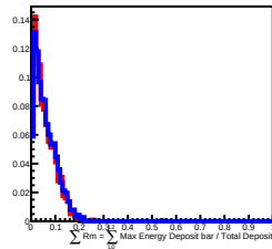
1000 GeV incident in L7
