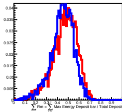
1000 GeV incident in L12
