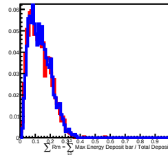
1000 GeV incident in L8
