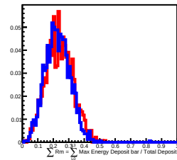
100 GeV incident in L8
