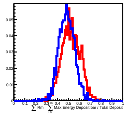
100 GeV incident in L10
