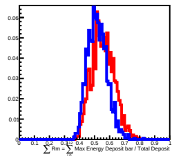
100 GeV incident in L12
