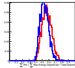
100 GeV incident in L13
