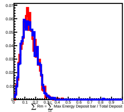
100 GeV incident in L7
