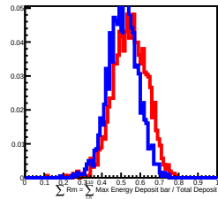
200 GeV incident in L10
