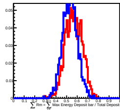
200 GeV incident in L11
