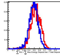
200 GeV incident in L9
