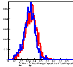
30 GeV incident in L9
