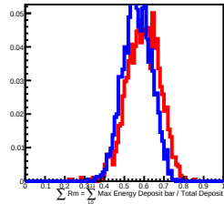
400 GeV incident in L11
