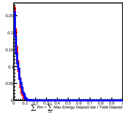
400 GeV incident in L6
