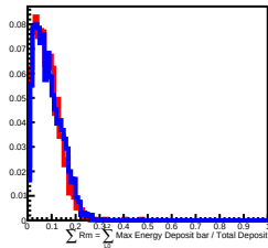
400 GeV incident in L7
