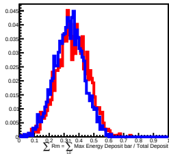
400 GeV incident in L10
