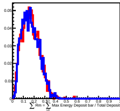
400 GeV incident in L8
