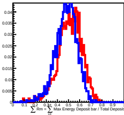
400 GeV incident in L13
