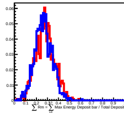
40 GeV incident in L8
