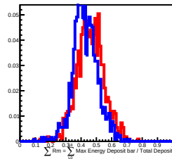
40 GeV incident in L13
