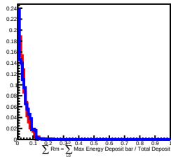
40 GeV incident in L5
