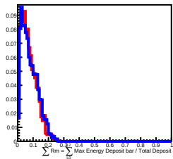
500 GeV incident in L7
