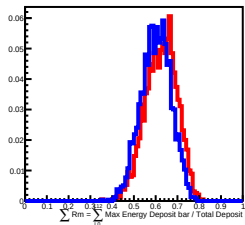
500 GeV incident in L12
