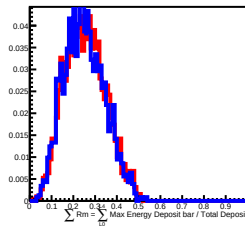
500 GeV incident in L9
