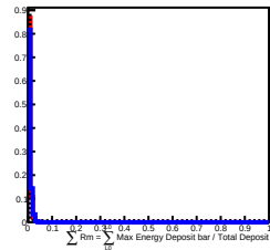
500 GeV incident in L5
