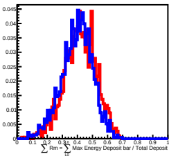
500 GeV incident in L11
