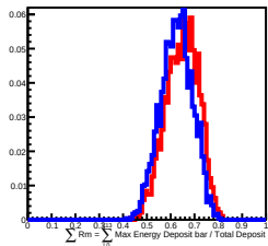
500 GeV incident in L13
