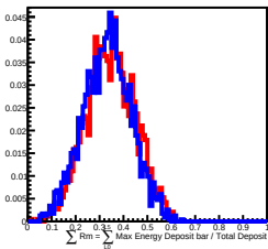
500 GeV incident in L10
