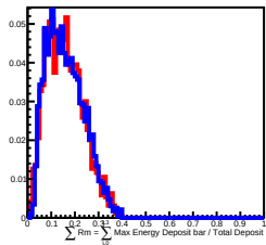
500 GeV incident in L8
