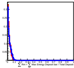
500 GeV incident in L6
