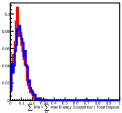
50 GeV incident in L6
