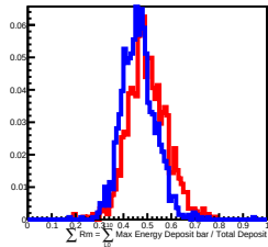
50 GeV incident in L10
