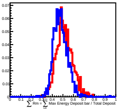
50 GeV incident in L11
