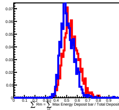
50 GeV incident in L13
