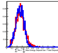
50 GeV incident in L8
