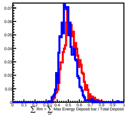
50 GeV incident in L12
