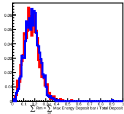
50 GeV incident in L7
