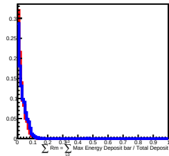
50 GeV incident in L5
