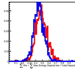
50 GeV incident in L9
