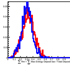
60 GeV incident in L9
