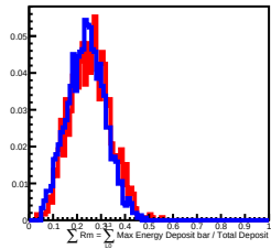
70 GeV incident in L8
