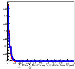
70 GeV incident in L5
