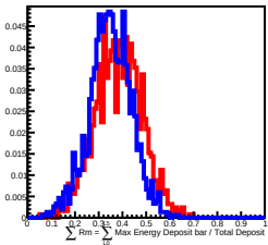
70 GeV incident in L10
