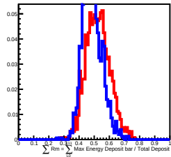
70 GeV incident in L11
