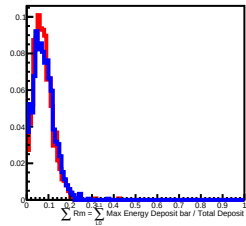
70 GeV incident in L6
