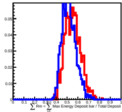
70 GeV incident in L13
