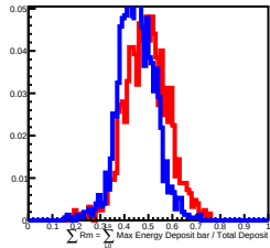
70 GeV incident in L9
