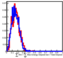
70 GeV incident in L7
