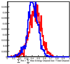
70 GeV incident in L12
