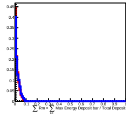
800 GeV incident in L6
