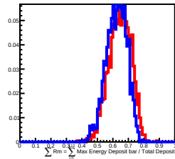
800 GeV incident in L12
