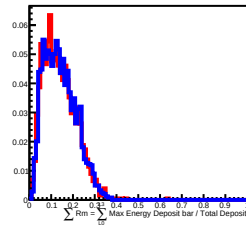
800 GeV incident in L8
