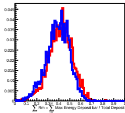
800 GeV incident in L11
