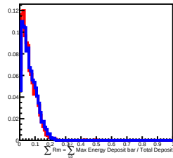
800 GeV incident in L7
