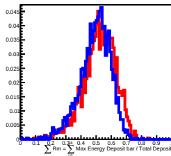
800 GeV incident in L13
