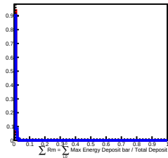
800 GeV incident in L5
