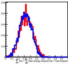
800 GeV incident in L10
