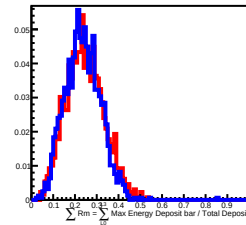
80 GeV incident in L8
