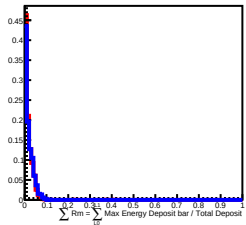
900 GeV incident in L6
