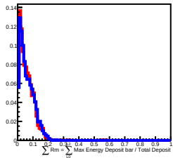
900 GeV incident in L7
