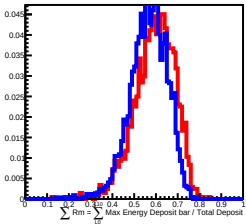
900 GeV incident in L10
