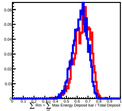
900 GeV incident in L12
