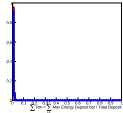
900 GeV incident in L5
