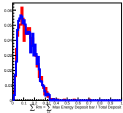
900 GeV incident in L8
