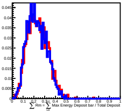
900 GeV incident in L9
