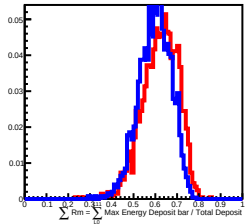
900 GeV incident in L11
