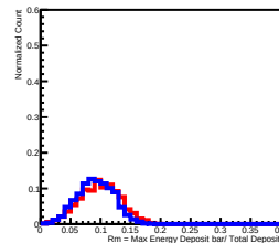
700 GeV incident in L4
