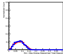
700 GeV incident in L3
