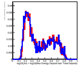
Deposit Energy[1000.00GeV, 1584.89GeV] in L5
