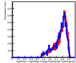
Deposit Energy[1000.00GeV, 1584.89GeV] in L10
