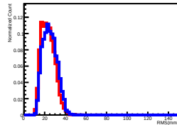
Deposit Energy[1000.00GeV, 1584.89GeV] in L9
