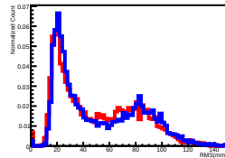
Deposit Energy[1000.00GeV, 1584.89GeV] in L2
