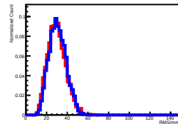
Deposit Energy[1000.00GeV, 1584.89GeV] in L13
