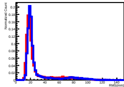
Deposit Energy[1000.00GeV, 1584.89GeV] in L5
