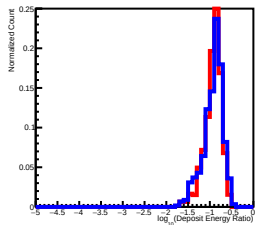
Deposit Energy[10.00GeV, 15.85GeV] EdgeRatio Distribution in L1
