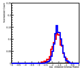
Deposit Energy[39.81GeV, 63.10GeV] EdgeRatio Distribution in L13
