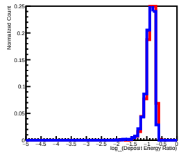
Deposit Energy[39.81GeV, 63.10GeV] EdgeRatio Distribution in L3
