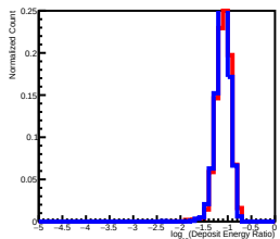
Deposit Energy[39.81GeV, 63.10GeV] EdgeRatio Distribution in L6
