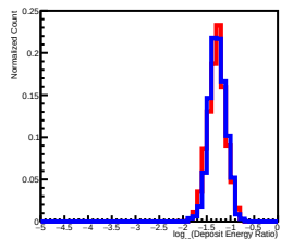
Deposit Energy[39.81GeV, 63.10GeV] EdgeRatio Distribution in L8
