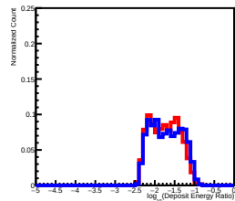
Deposit Energy[39.81GeV, 63.10GeV] EdgeRatio Distribution in L0
