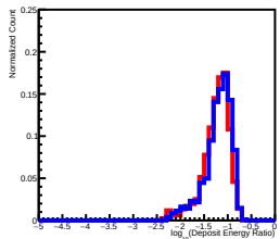
Deposit Energy[39.81GeV, 63.10GeV] EdgeRatio Distribution in L1
