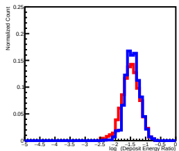
Deposit Energy[39.81GeV, 63.10GeV] EdgeRatio Distribution in L11
