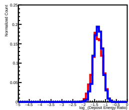
Deposit Energy[39.81GeV, 63.10GeV] EdgeRatio Distribution in L9
