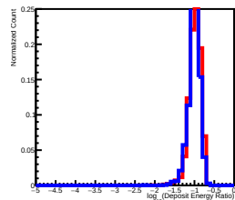
Deposit Energy[39.81GeV, 63.10GeV] EdgeRatio Distribution in L5
