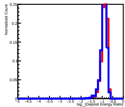
Deposit Energy[39.81GeV, 63.10GeV] EdgeRatio Distribution in L4
