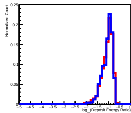
Deposit Energy[398.11GeV, 630.96GeV] EdgeRatio Distribution in L3
