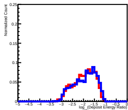
Deposit Energy[398.11GeV, 630.96GeV] EdgeRatio Distribution in L1
