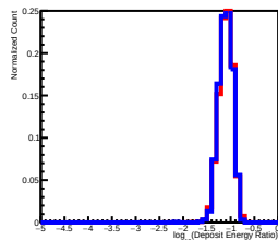
Deposit Energy[398.11GeV, 630.96GeV] EdgeRatio Distribution in L8
