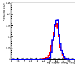
Deposit Energy[398.11GeV, 630.96GeV] EdgeRatio Distribution in L13
