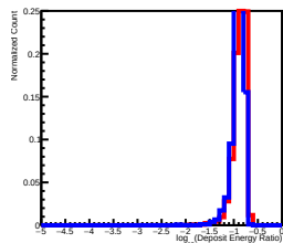
Deposit Energy[398.11GeV, 630.96GeV] EdgeRatio Distribution in L5
