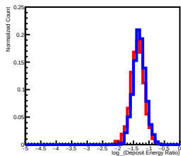
Deposit Energy[398.11GeV, 630.96GeV] EdgeRatio Distribution in L11
