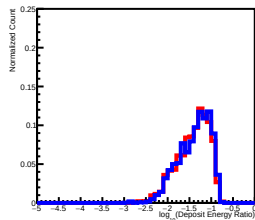
Deposit Energy[398.11GeV, 630.96GeV] EdgeRatio Distribution in L2
