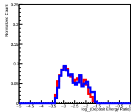
Deposit Energy[398.11GeV, 630.96GeV] EdgeRatio Distribution in L0
