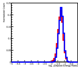
Deposit Energy[398.11GeV, 630.96GeV] EdgeRatio Distribution in L10
