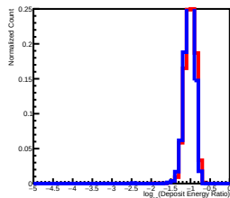
Deposit Energy[398.11GeV, 630.96GeV] EdgeRatio Distribution in L7
