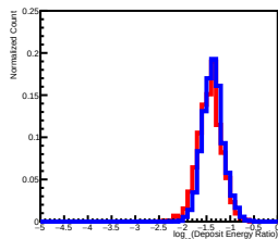
Deposit Energy[398.11GeV, 630.96GeV] EdgeRatio Distribution in L12
