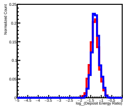
Deposit Energy[1584.89GeV, 2511.89GeV] EdgeRatio Distribution in L11
