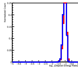
Deposit Energy[1584.89GeV, 2511.89GeV] EdgeRatio Distribution in L8
