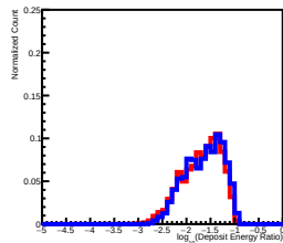
Deposit Energy[1584.89GeV, 2511.89GeV] EdgeRatio Distribution in L7
