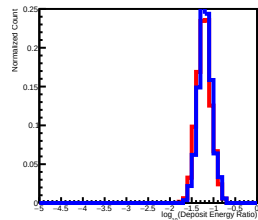
Deposit Energy[1584.89GeV, 2511.89GeV] EdgeRatio Distribution in L10
