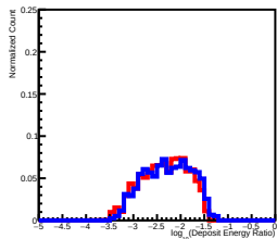
Deposit Energy[1584.89GeV, 2511.89GeV] EdgeRatio Distribution in L6
