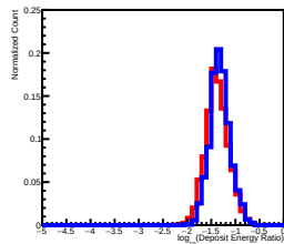
Deposit Energy[1584.89GeV, 2511.89GeV] EdgeRatio Distribution in L12
