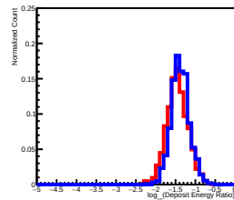
Deposit Energy[1584.89GeV, 2511.89GeV] EdgeRatio Distribution in L13
