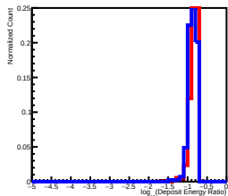
Deposit Energy[3981.07GeV, 6309.57GeV] EdgeRatio Distribution in L6
