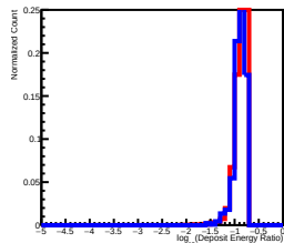
Deposit Energy[3981.07GeV, 6309.57GeV] EdgeRatio Distribution in L5
