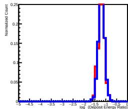
Deposit Energy[3981.07GeV, 6309.57GeV] EdgeRatio Distribution in L10
