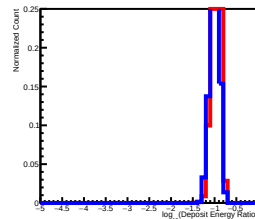
Deposit Energy[3981.07GeV, 6309.57GeV] EdgeRatio Distribution in L8
