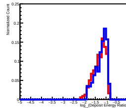
Deposit Energy[3981.07GeV, 6309.57GeV] EdgeRatio Distribution in L3
