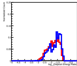
Deposit Energy[3981.07GeV, 6309.57GeV] EdgeRatio Distribution in L2
