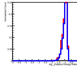
Deposit Energy[3981.07GeV, 6309.57GeV] EdgeRatio Distribution in L4
