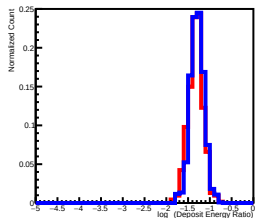
Deposit Energy[3981.07GeV, 6309.57GeV] EdgeRatio Distribution in L11
