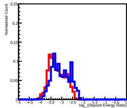
Deposit Energy[3981.07GeV, 6309.57GeV] EdgeRatio Distribution in L0
