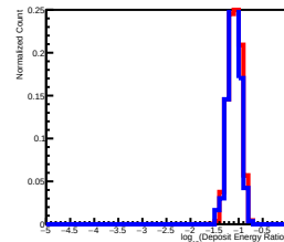
Deposit Energy[3981.07GeV, 6309.57GeV] EdgeRatio Distribution in L9
