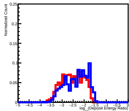
Deposit Energy[3981.07GeV, 6309.57GeV] EdgeRatio Distribution in L1
