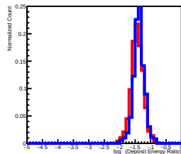
Deposit Energy[3981.07GeV, 6309.57GeV] EdgeRatio Distribution in L12
