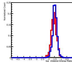
Deposit Energy[3981.07GeV, 6309.57GeV] EdgeRatio Distribution in L13
