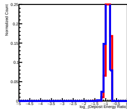
Deposit Energy[3981.07GeV, 6309.57GeV] EdgeRatio Distribution in L7
