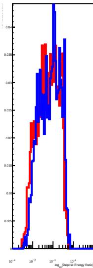
Deposit Energy(200.00GeV, 1584.89GeV)Deposited Energy Ratio
