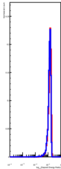
Deposit Energy(200.00GeV, 1584.89GeV)Deposited Energy Ratio
