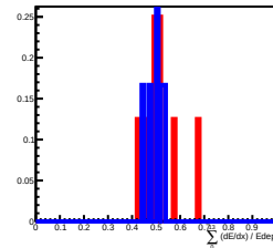
Deposit Energy[10.00GeV, 15.85GeV] in L13
