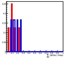
Deposit Energy[10.00GeV, 15.85GeV] in L6
