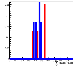
Deposit Energy[10.00GeV, 15.85GeV] in L9
