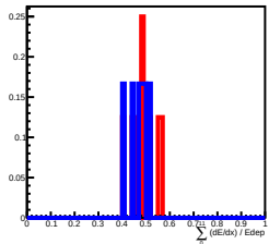
Deposit Energy[10.00GeV, 15.85GeV] in L11
