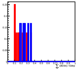
Deposit Energy[10.00GeV, 15.85GeV] in L7
