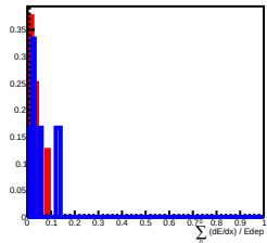
Deposit Energy[10.00GeV, 15.85GeV] in L5
