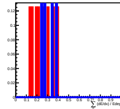
Deposit Energy[10.00GeV, 15.85GeV] in L8
