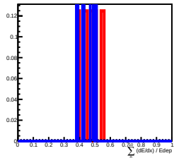
Deposit Energy[10.00GeV, 15.85GeV] in L10
