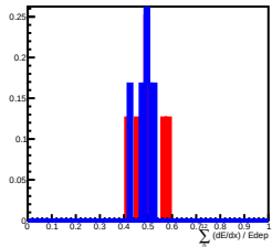
Deposit Energy[10.00GeV, 15.85GeV] in L12
