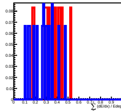
Deposit Energy[39.81GeV, 63.10GeV] in L9
