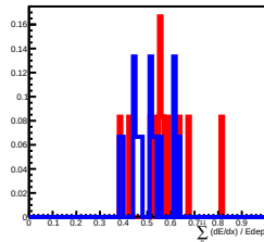
Deposit Energy[39.81GeV, 63.10GeV] in L1
