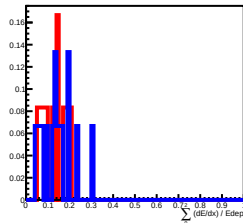
Deposit Energy[39.81GeV, 63.10GeV] in L7
