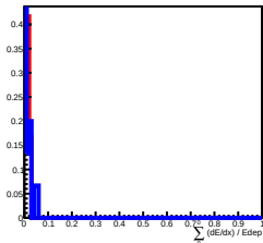
Deposit Energy[39.81GeV, 63.10GeV] in L5
