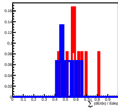
Deposit Energy[39.81GeV, 63.10GeV] in L12
