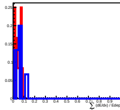
Deposit Energy[39.81GeV, 63.10GeV] in L6
