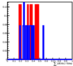
Deposit Energy[158.49GeV, 251.19GeV] in L10
