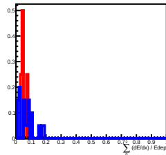
Deposit Energy[398.11GeV, 630.96GeV] in L7
