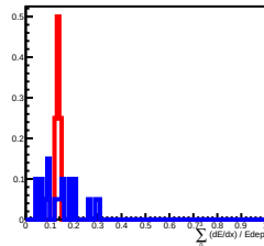
Deposit Energy[398.11GeV, 630.96GeV] in L8
