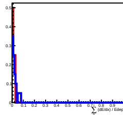
Deposit Energy[398.11GeV, 630.96GeV] in L6
