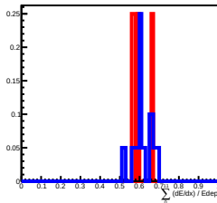
Deposit Energy[398.11GeV, 630.96GeV] in L11
