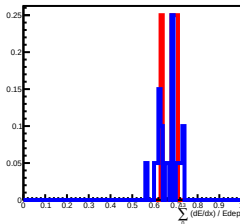
Deposit Energy[398.11GeV, 630.96GeV] in L13
