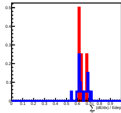
Deposit Energy[398.11GeV, 630.96GeV] in L12
