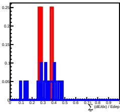
Deposit Energy[398.11GeV, 630.96GeV] in L10
