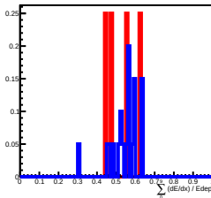
Deposit Energy[398.11GeV, 630.96GeV] in L9
