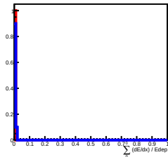
Deposit Energy[398.11GeV, 630.96GeV] in L5
